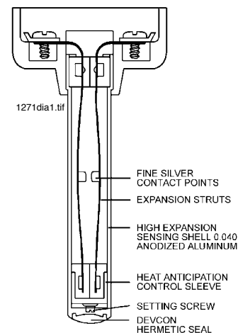
Cut-Away View
